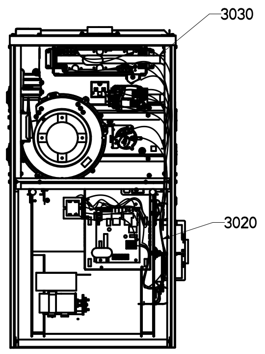
WIRE ROUTING
