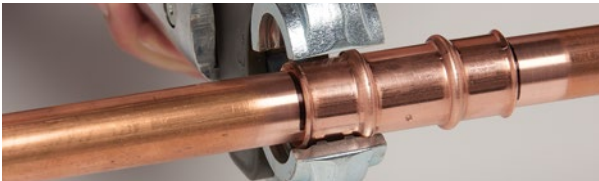
1. Insert the tube in the fitting
